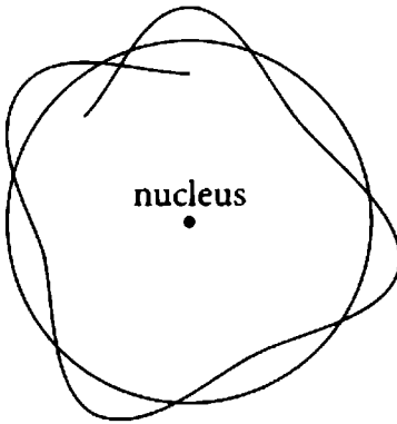
Forbidden orbit
