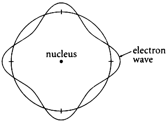
Allowed orbit
